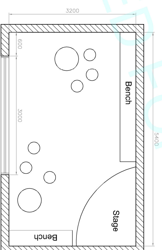
Floor Plan Scale 1:50
